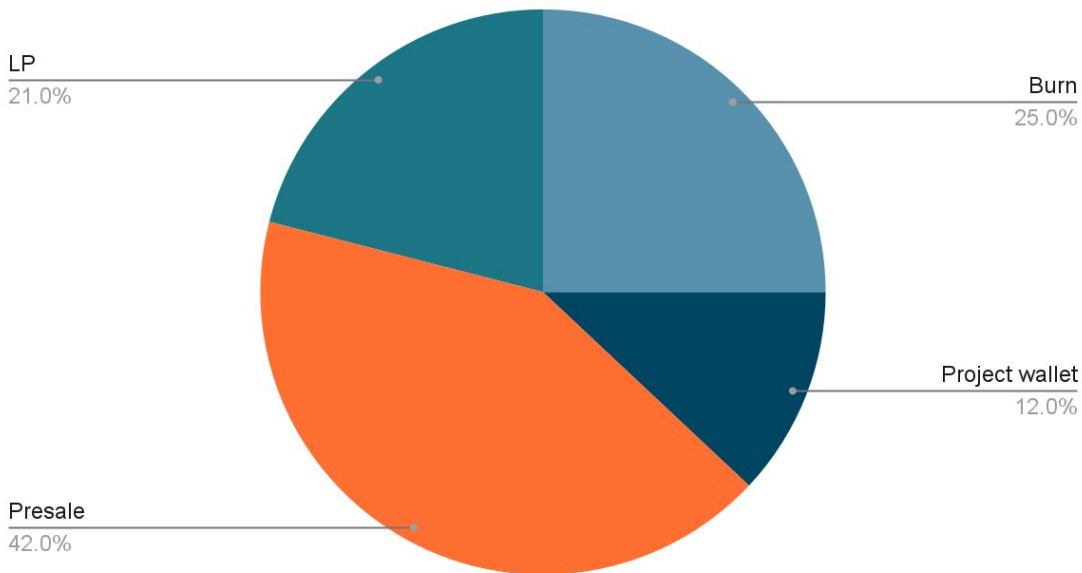
Token distribution
